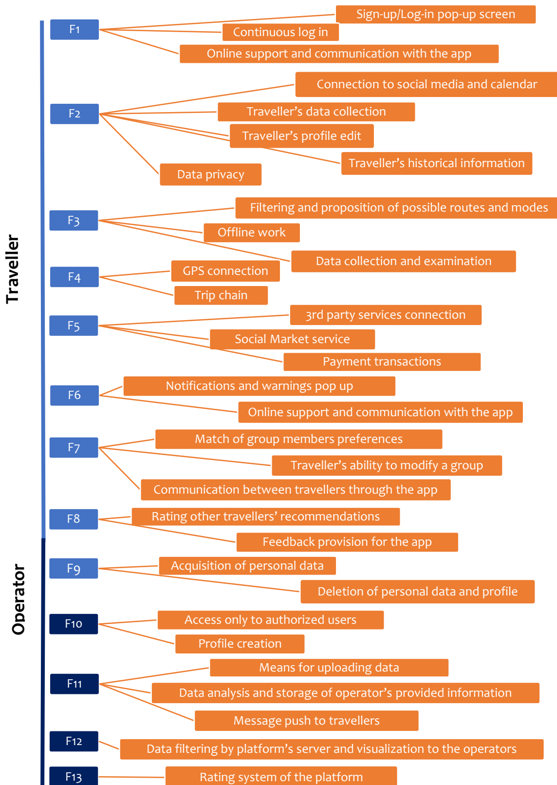
Figure 16: Elicitation of requirements
